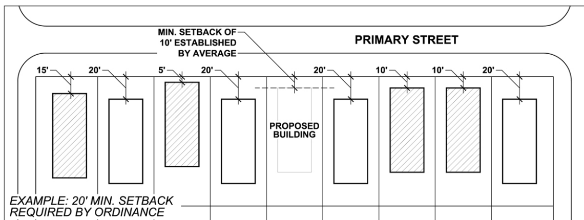
FIGURE 8-1: FRONT SETBACK AVERAGING
